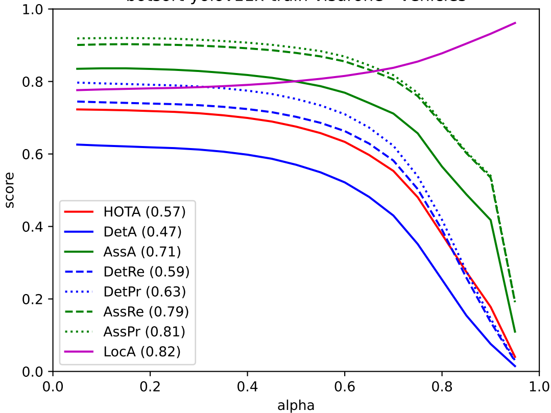
botsort-yolov11x-train-visdrone - vehicles
