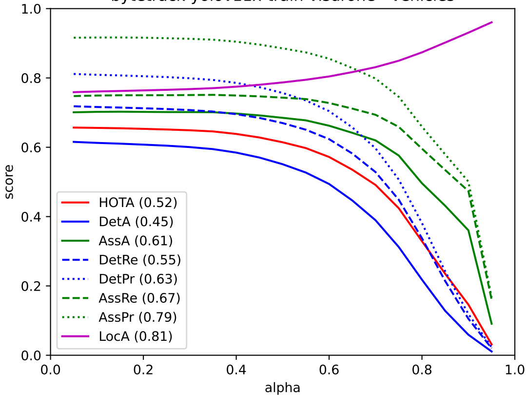
bytetrack-yolov11x-train-visdrone - vehicles
