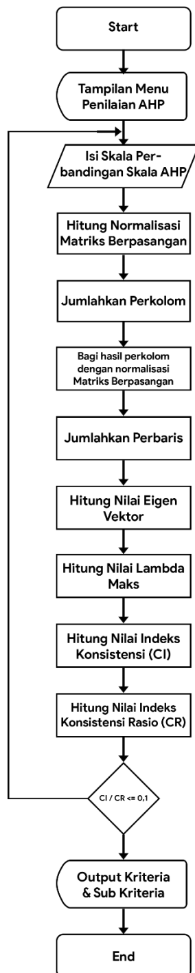
Gambar 4. Flowchart Perhitungan AHP
