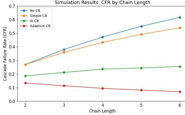
Figure 1: CFR increases with pipeline depth
