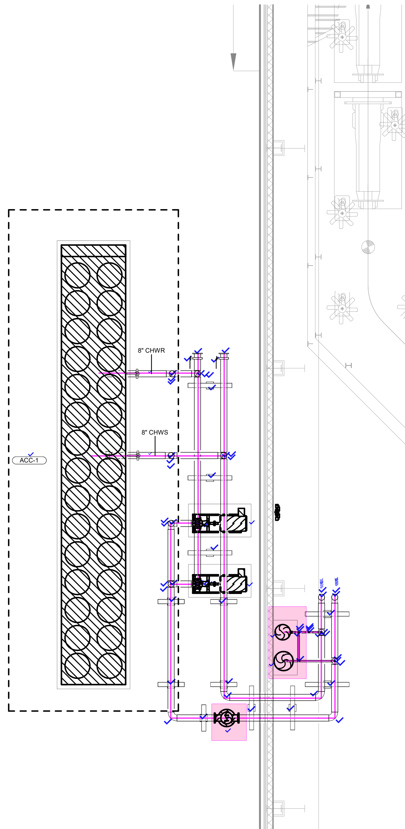
1 MECHANICAL ENLARGED PLAN - AREA C CHILLER 1 3/16" = 1'-0"
