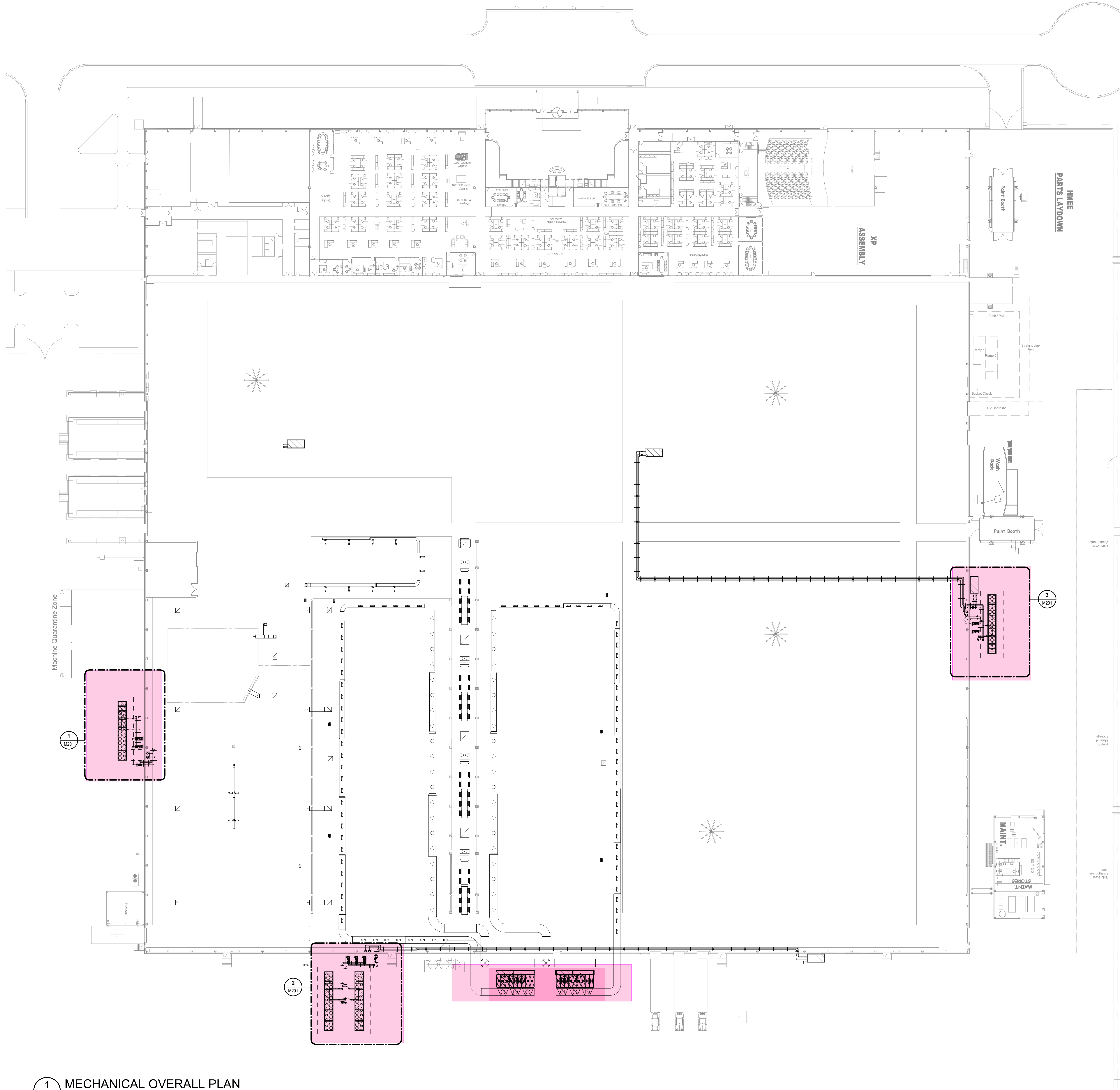
1 MECHANICAL OVERALL PLAN M111 1" = 30'-0"
