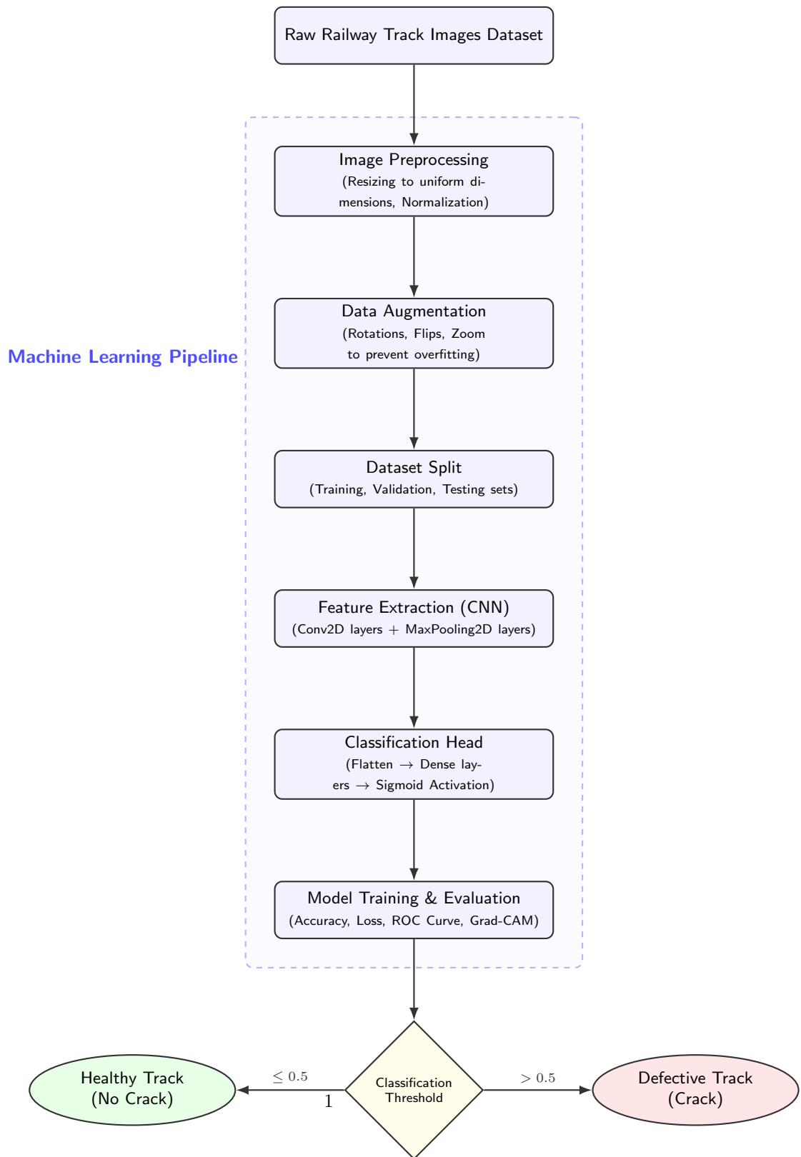
Figure 1: Proposed methodology and workflow for automated railway track crack detection.
