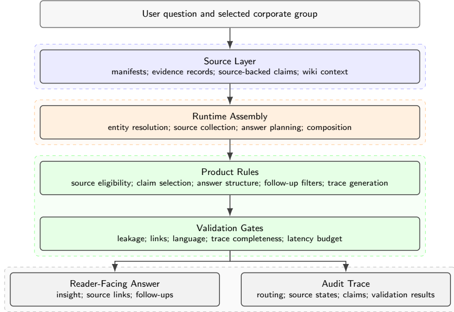
Figure 1: Traceable LLM-agent harness. The architecture separates source authority, runtime assembly, product rules, validation gates, and two outputs: a reader-facing answer and an audit trace.
