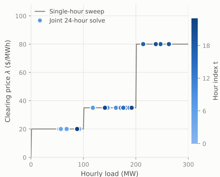
(c) Clearing Price Against Hourly Load
