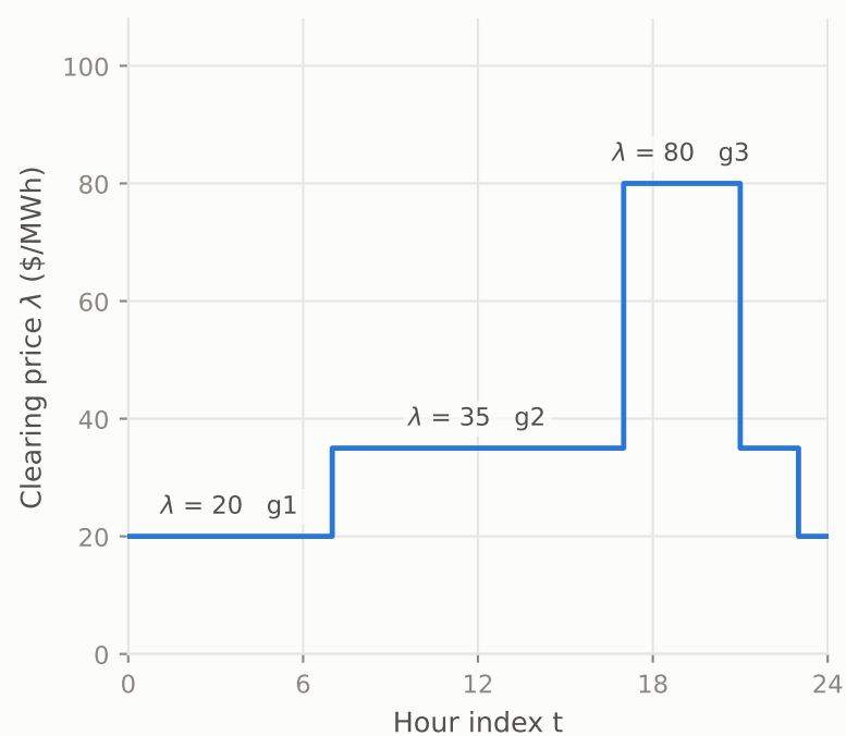
(b) Clearing Price by Hour
