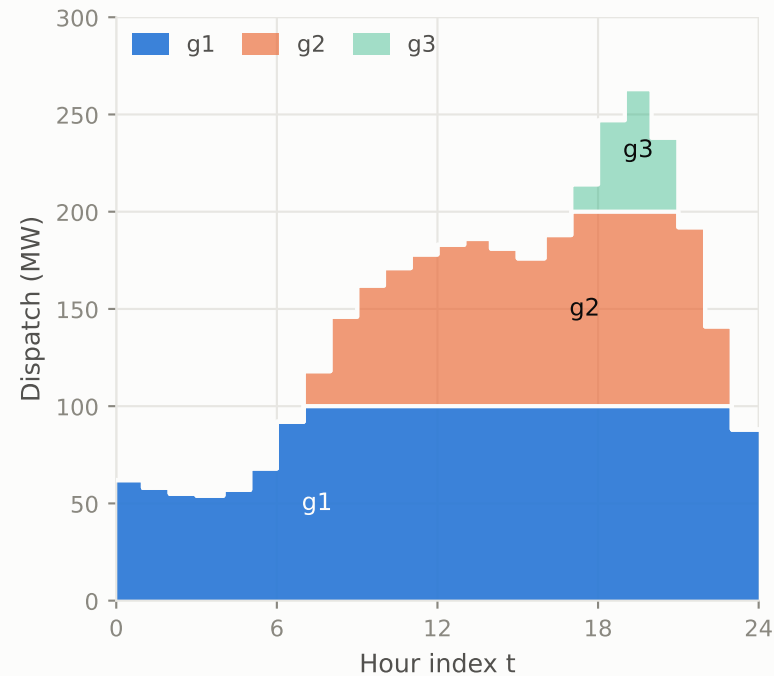
(a) Dispatch by Hour, in Merit Order
