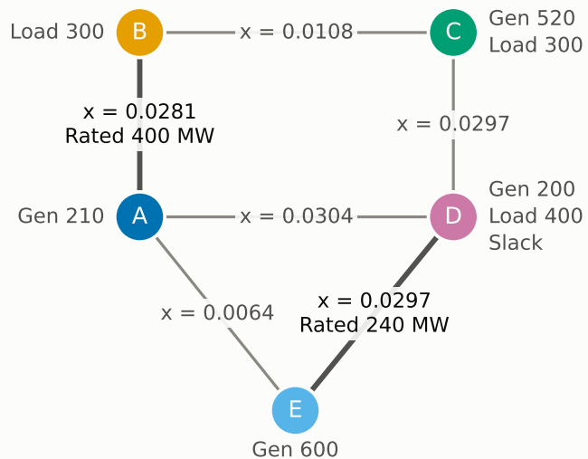
(a) Network, Capacity and Load (MW)
