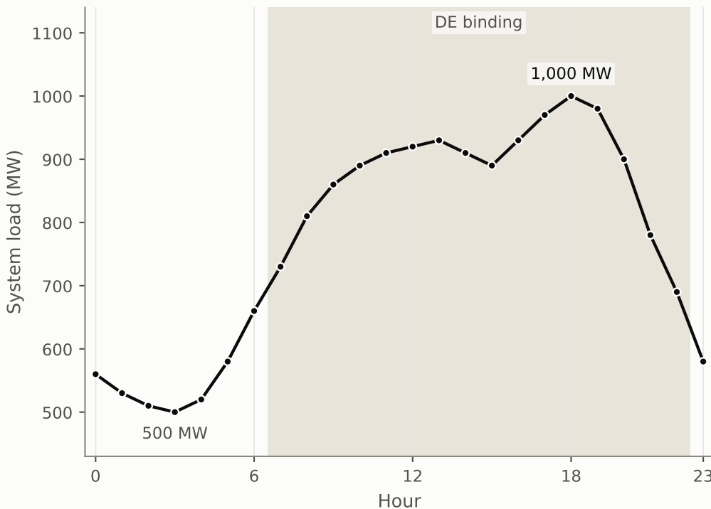
(a) System Load Across the Day
