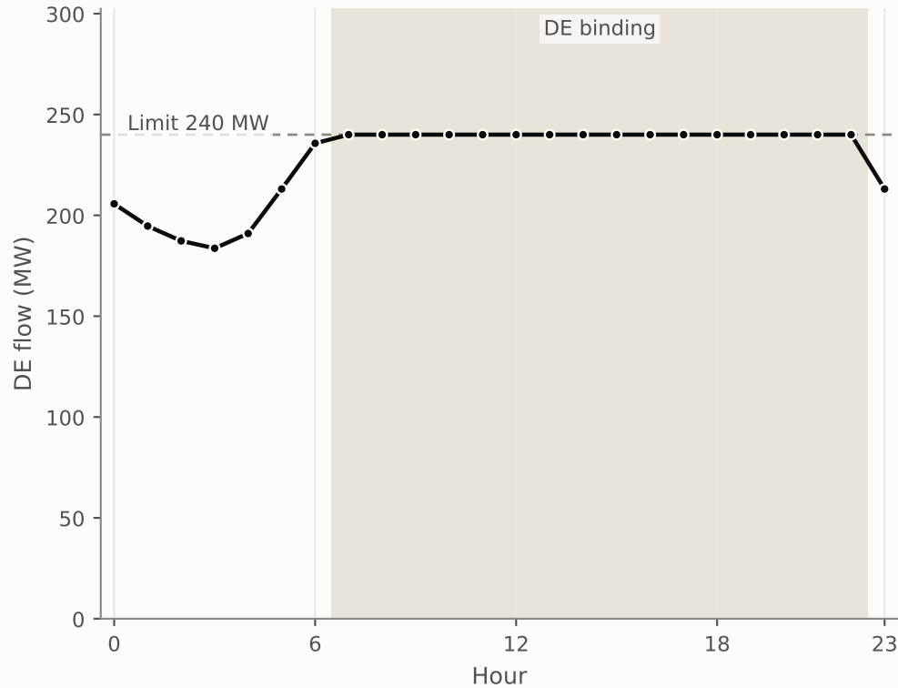
(b) The DE Corridor Against Its Limit
