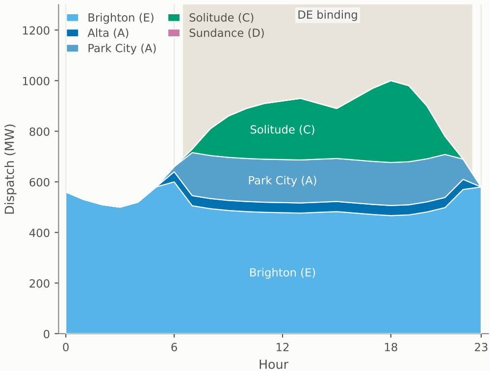
(a) Dispatch by Unit, Stacked in Merit Order
