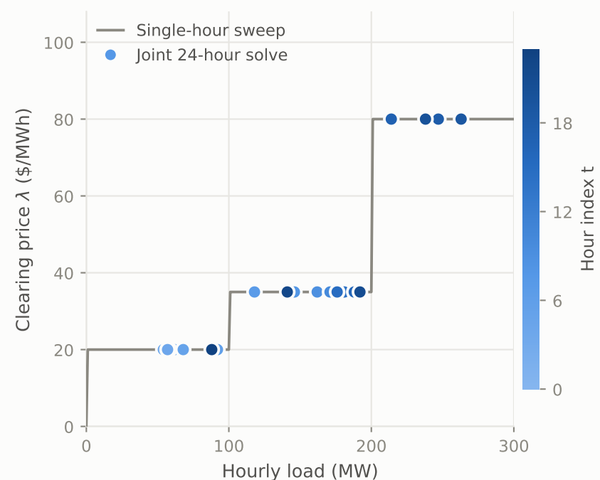
(c) Clearing price against hourly load
