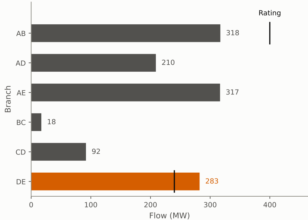
(b) Flow against rating
