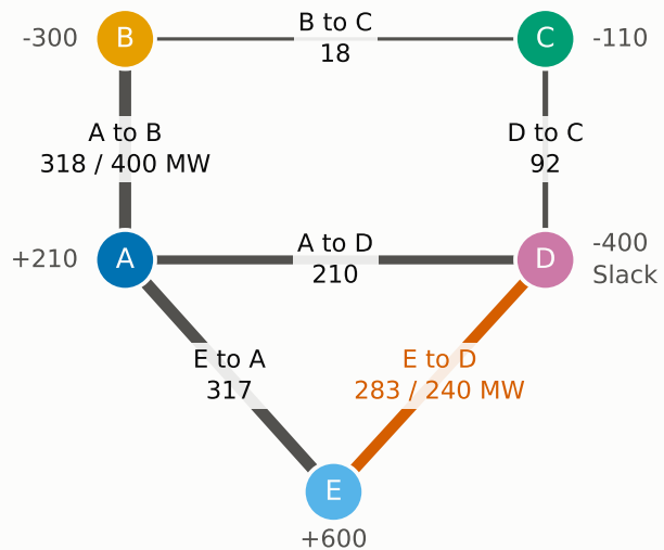
(a) Flows and net injection (MW)
