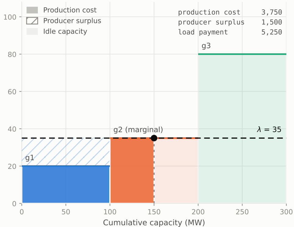
(a) Supply stack at D = 150 MW
