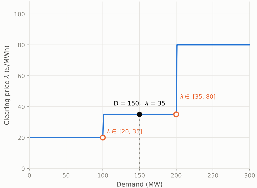
(b) Clearing price against demand
