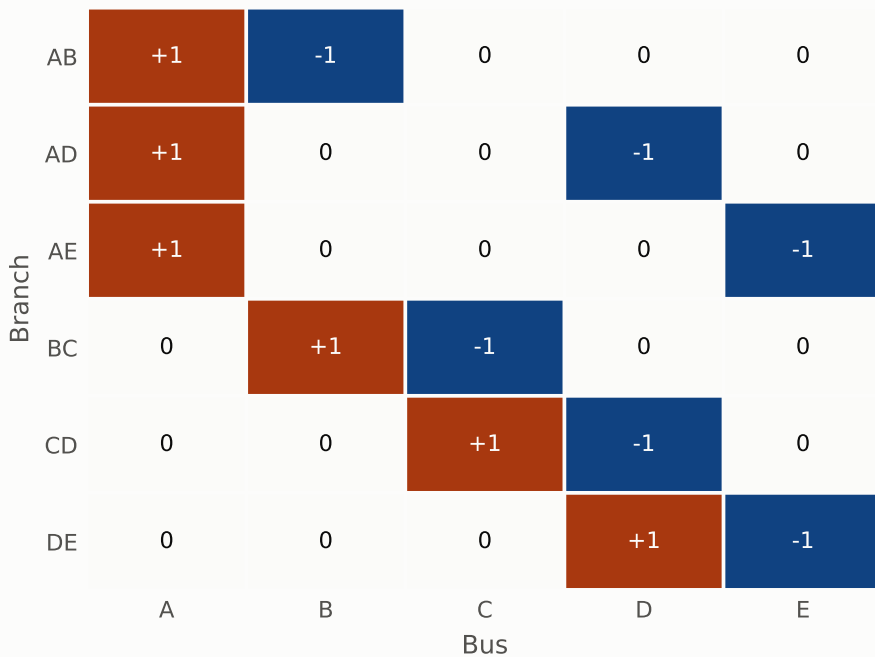
(a) Branch-bus incidence A
