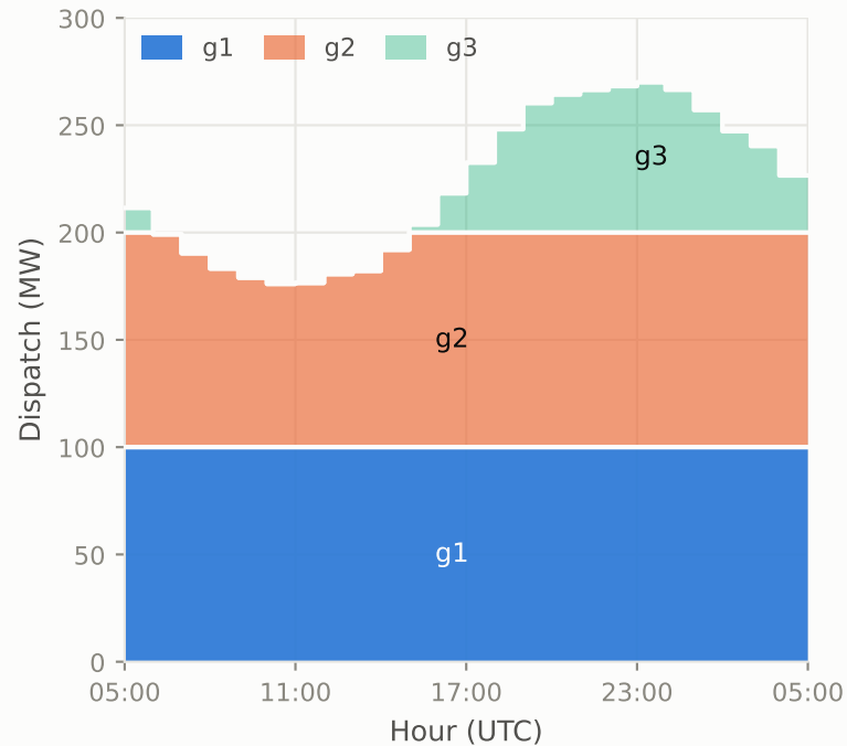
(b) Dispatch by hour, in merit order
