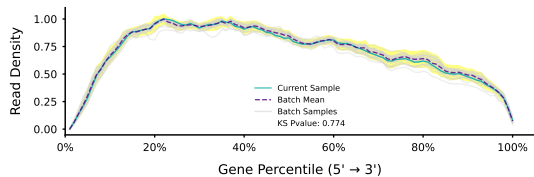
GeneBody Coverage
