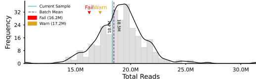
Alignment
