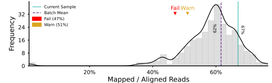
Sequence Contamination
