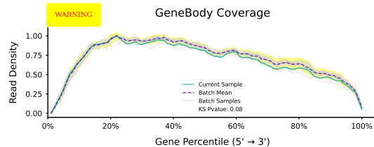
GeneBody Coverage
