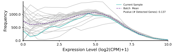
Gene Expression
