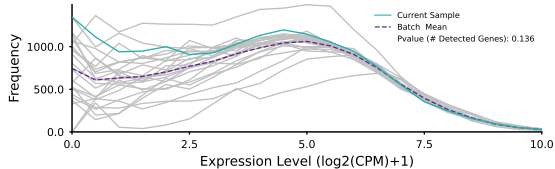
Gene Expression
