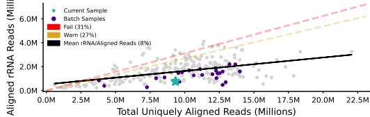
Gene Expression
