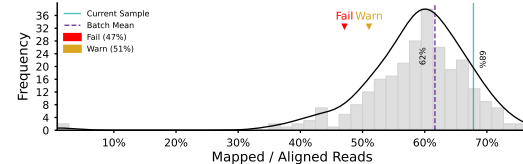
Sequence Contamination
