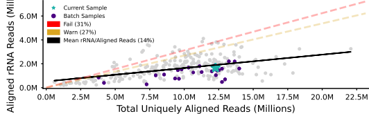
Gene Expression
