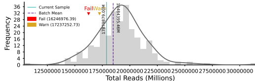
Alignment
