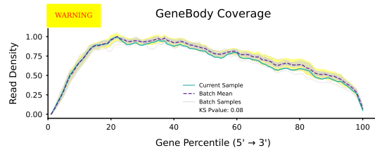
GeneBody Coverage
