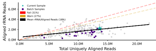
Gene Expression
