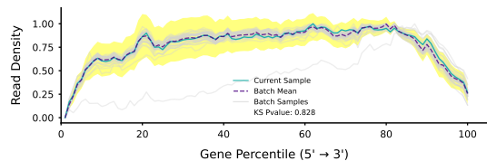
GeneBody Coverage
