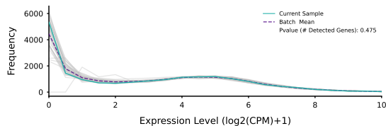
Gene Expression
