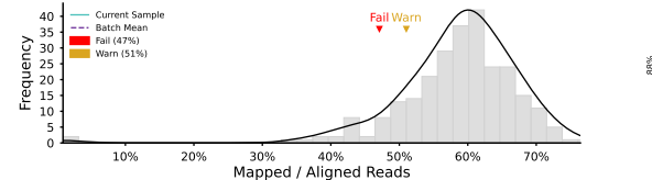
Sequence Contamination
