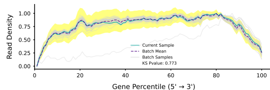
GeneBody Coverage
