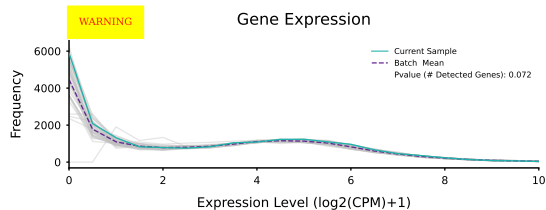
Gene Expression
