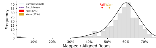
Sequence Contamination
