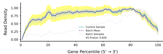
GeneBody Coverage
