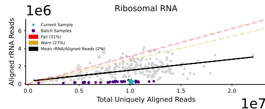
Gene Expression
