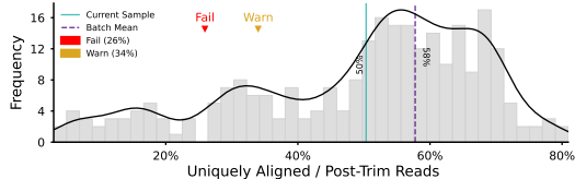
Alignment
