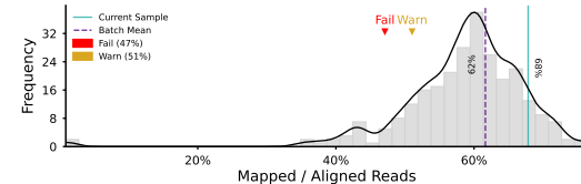
Exon Mapping
