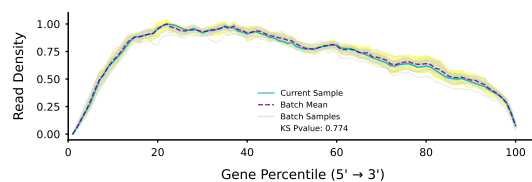
GeneBody Coverage
