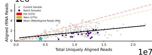
Gene Expression
