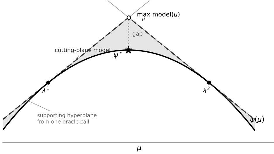
Figure 4.1: The horizontal axis is \mu , the free variable of the inequality above. Here \lambda^1 and \lambda^2 are the two points at which the oracle has been called, and the drawing is the one-dimensional case, so that the supporting hyperplanes appear as lines. One oracle call at \lambda returns \psi(\lambda) and a supergradient, and hence a hyperplane that lies above \psi everywhere , not merely near \lambda : this is what concavity buys. The model is the pointwise minimum of the hyperplanes collected so far, so it too lies above \psi , and its maximum is an upper bound on \psi^* . Each new call adds a hyperplane, which can only lower the minimum. The method probes next where the model is highest, since that is the only place the maximum can be.
