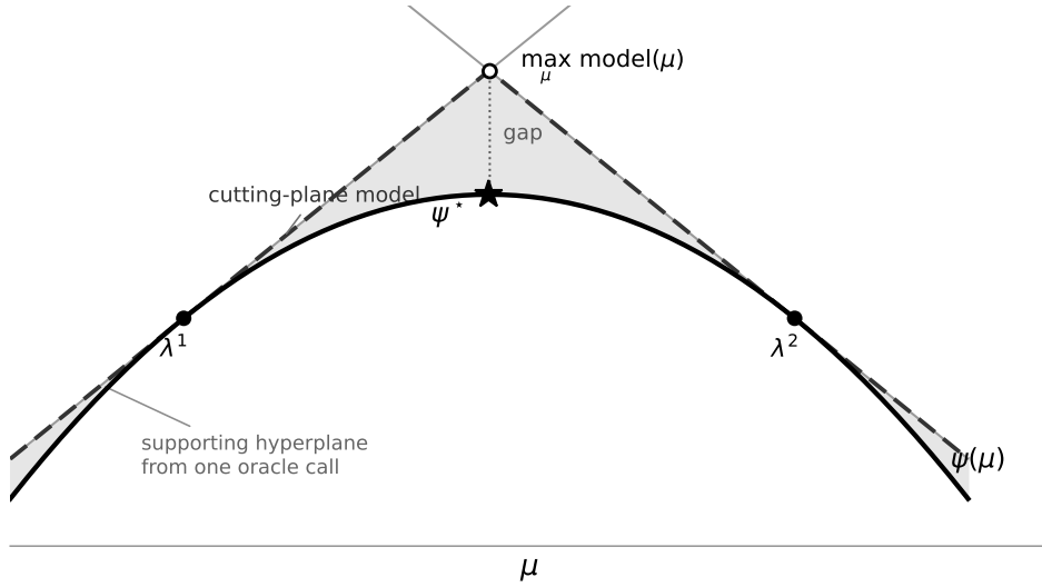
Figure 5.1: The horizontal axis is \mu , the free variable of the inequality above. Here \lambda^1 and \lambda^2 are the two points at which the oracle has been called, and the drawing is the one-dimensional case, so that the supporting hyperplanes appear as lines. One oracle call at \lambda returns \psi(\lambda) and a supergradient, and hence a hyperplane that lies above \psi everywhere , not merely near \lambda : this is what concavity buys. The model is the pointwise minimum of the hyperplanes collected so far, so it too lies above \psi , and its maximum is an upper bound on \psi^* . Each new call adds a hyperplane, which can only lower the minimum. The method probes next where the model is highest, since that is the only place the maximum can be.
