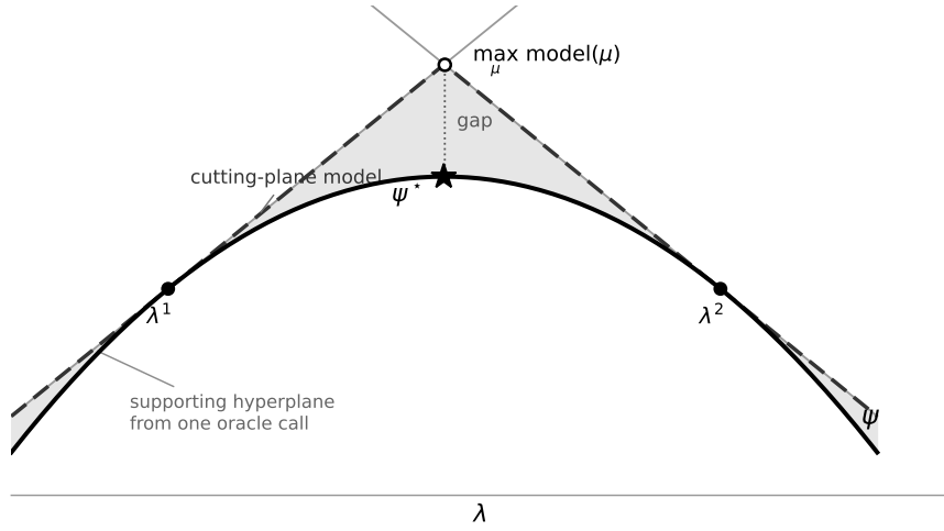
Figure 4.1: One oracle call at \lambda returns \psi(\lambda) and a supergradient, and hence a hyperplane that lies above \psi everywhere , not merely near \lambda : this is what concavity buys. The model is the pointwise minimum of the hyperplanes collected so far, so it too lies above \psi , and its maximum is an upper bound on \psi^* . Each new call adds a hyperplane, which can only lower the minimum; the method probes next where the model is highest, since that is the only place the maximum can be.
