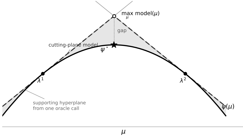
Figure 4.1: The horizontal axis is \mu , the free variable of the inequality above. Here \lambda^1 and \lambda^2 are the two points at which the oracle has been called, and the drawing is the one-dimensional case, so that the supporting hyperplanes appear as lines. One oracle call at \lambda returns \psi(\lambda) and a supergradient, and hence a hyperplane that lies above \psi everywhere , not merely near \lambda : this is what concavity buys. The model is the pointwise minimum of the hyperplanes collected so far, so it too lies above \psi , and its maximum is an upper bound on \psi^* . Each new call adds a hyperplane, which can only lower the minimum. The method probes next where the model is highest, since that is the only place the maximum can be.
