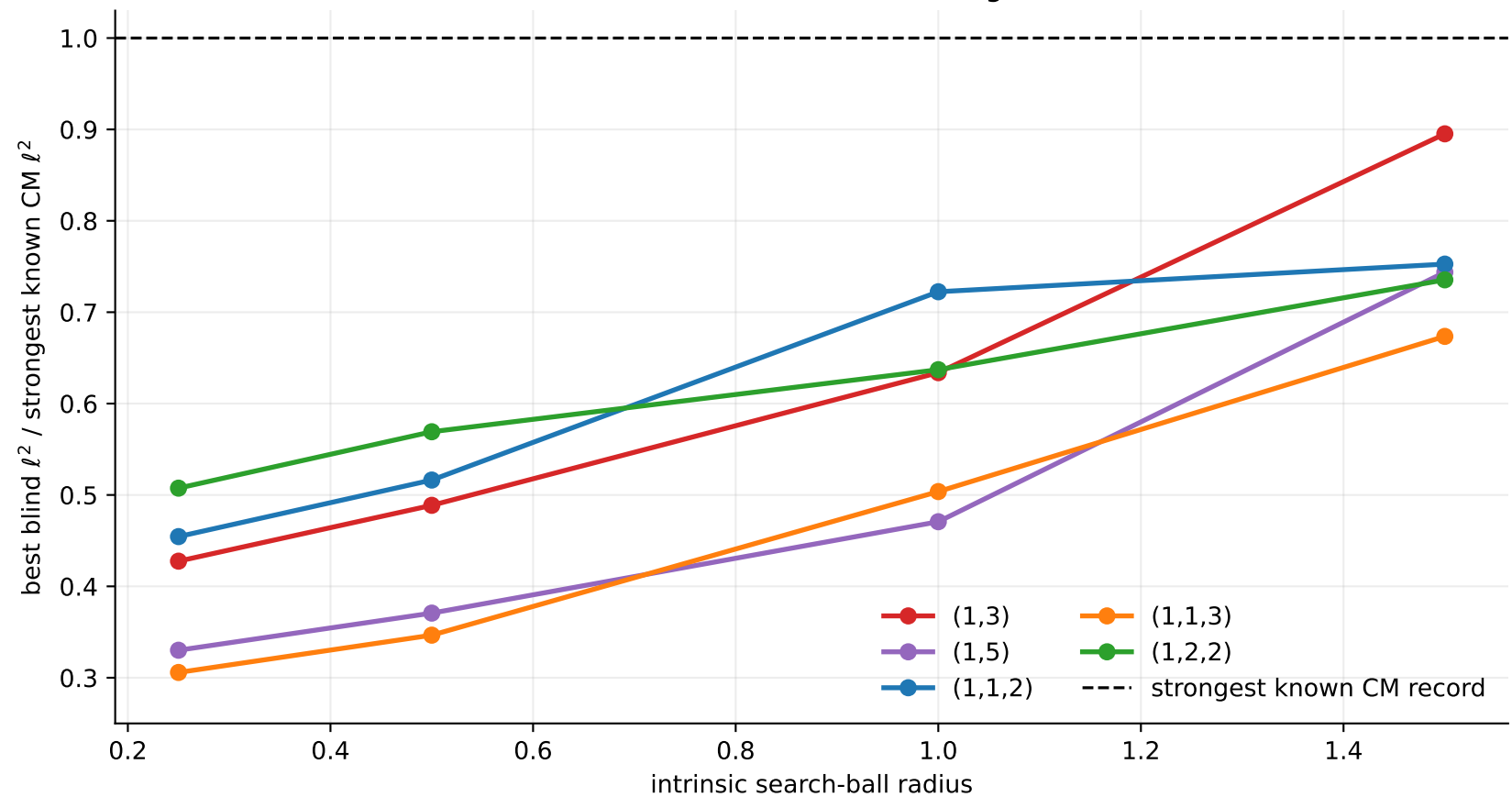
Blind bounded search does not reach the strongest known CM records
