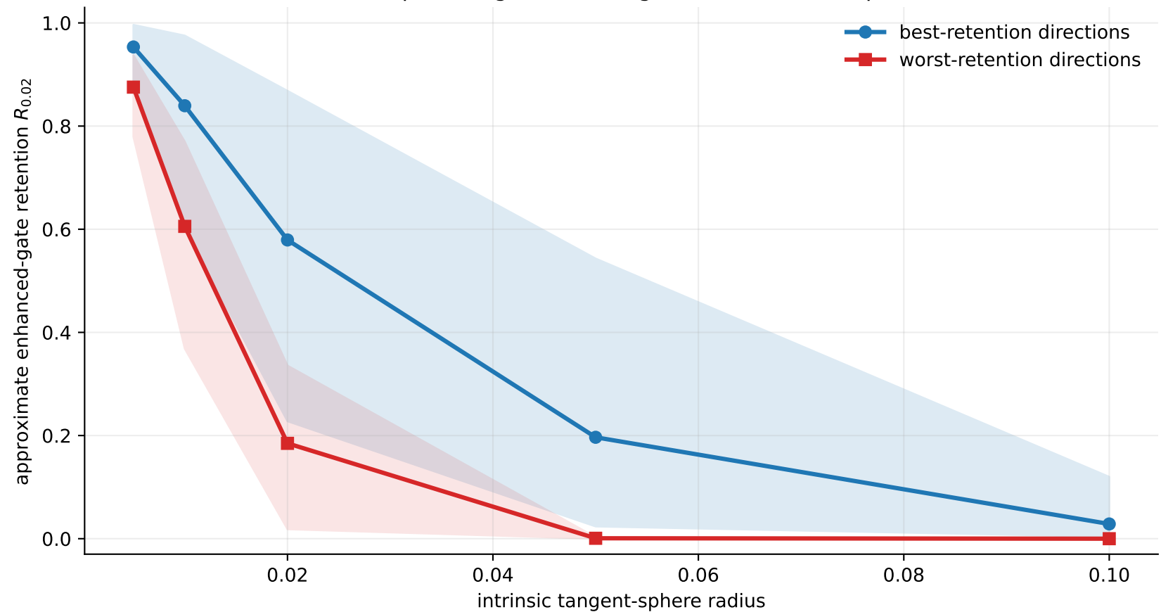
Enhanced passive gates are fragile but direction-dependent
