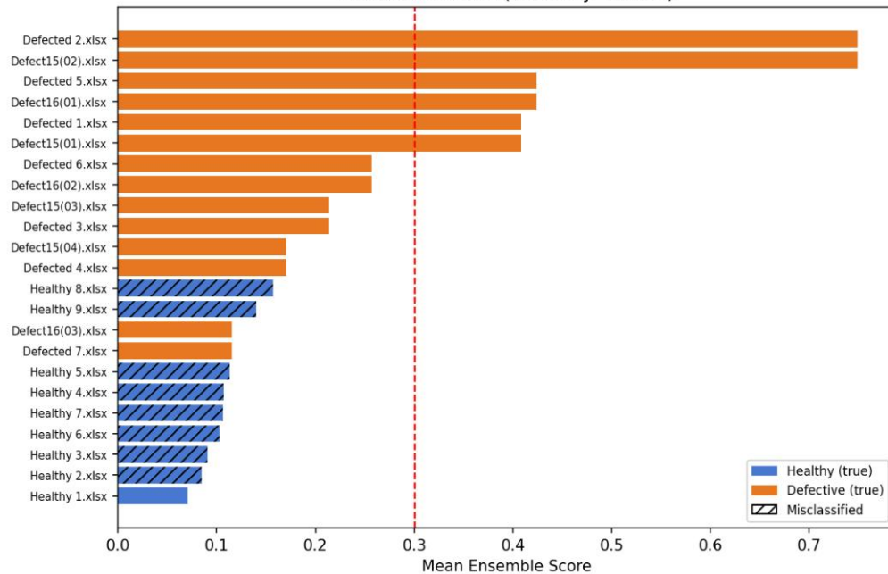
File Classification (accuracy=65.2%)
