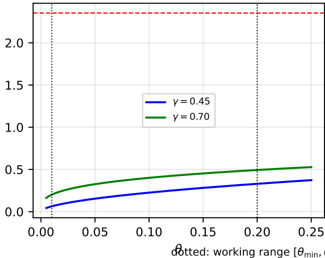
\theta\phi(\theta) : sup at \theta_{\max} always
