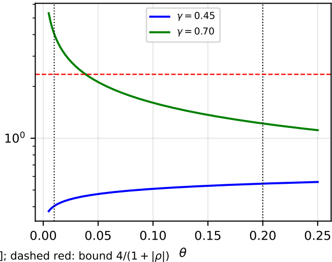
\theta\phi(\theta)^2 : sup at endpoint depending on \gamma \lesssim \frac{1}{2}
