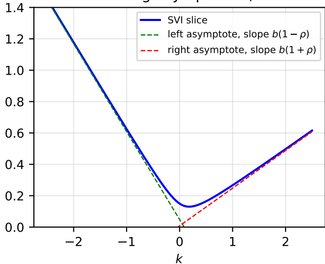
SVI slice and wing asymptotes (Lee bounds)
