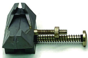
Plastic Case Holder
