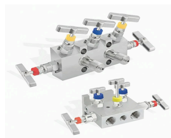
5 Valve Instrumentation Manifold
