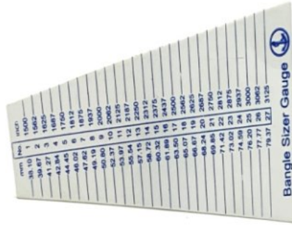
BANGLE SIZE GAUGE
