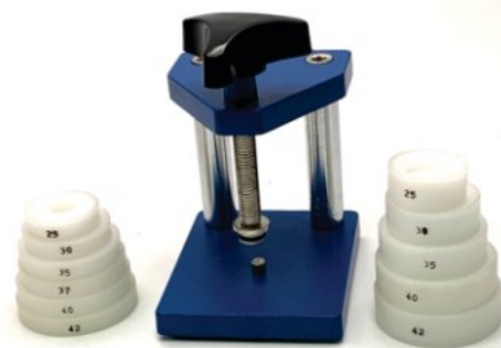
GLASS FITTING MACHINE OLD MODEL
