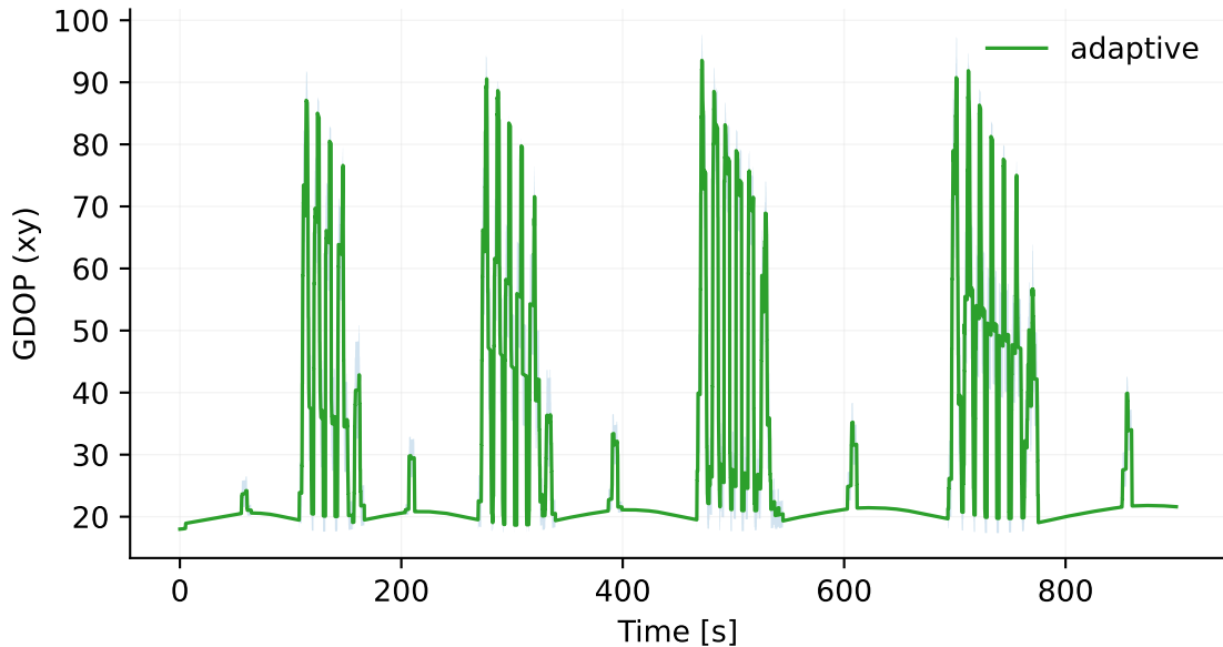
GDOP vs time (adaptive policies)
