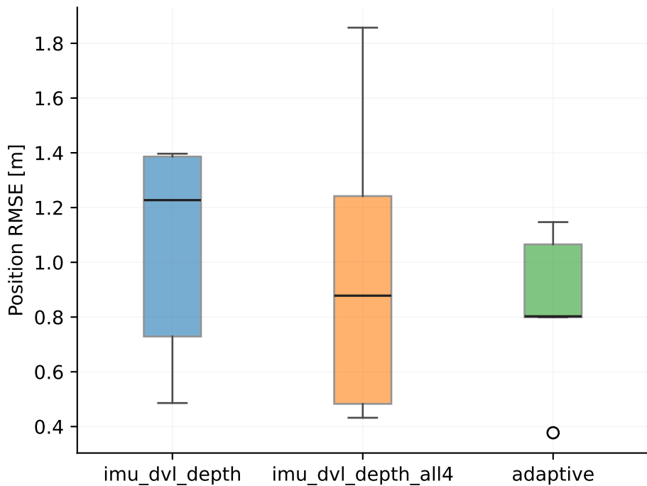
RMSE by algorithm
