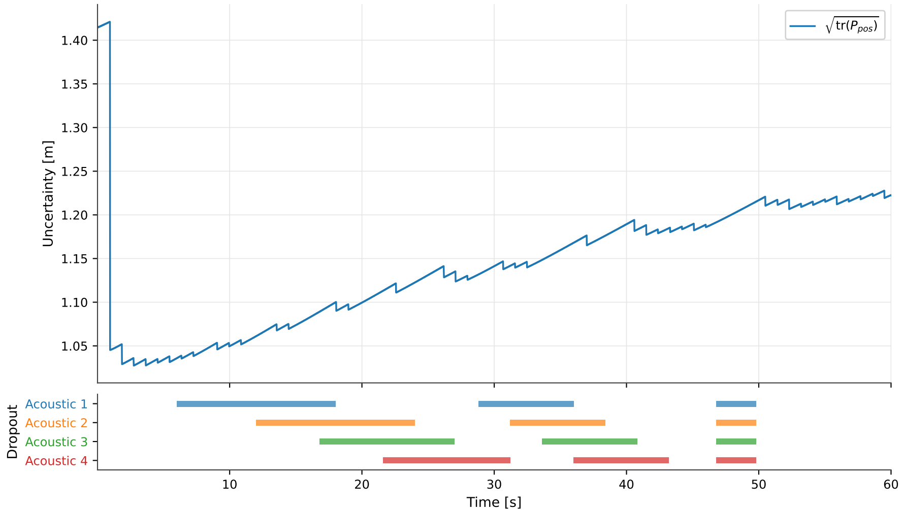
Position uncertainty with modem dropout timeline
