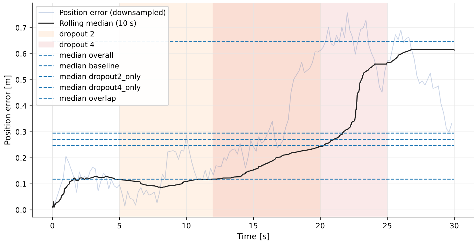
Position error with rolling median
