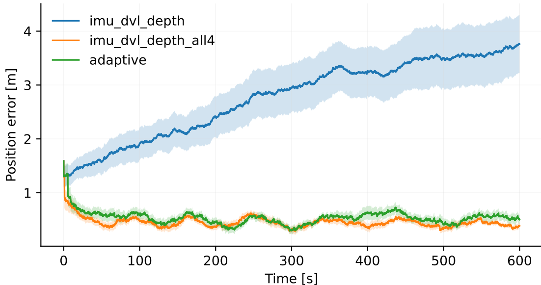
Position error vs time (mean \pm 95% CI)
