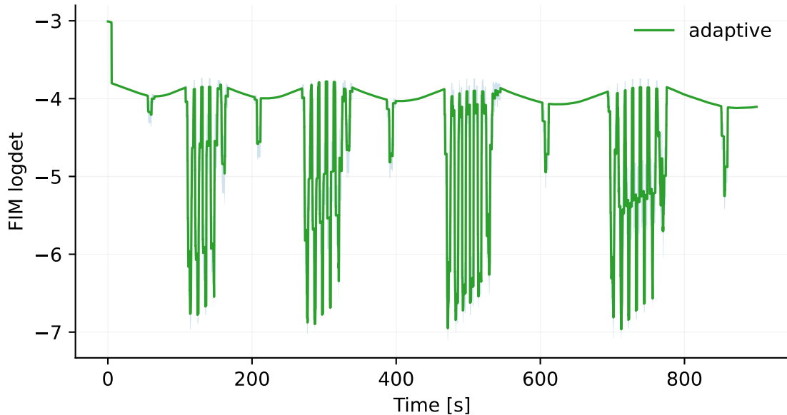
FIM logdet vs time (adaptive policies)
