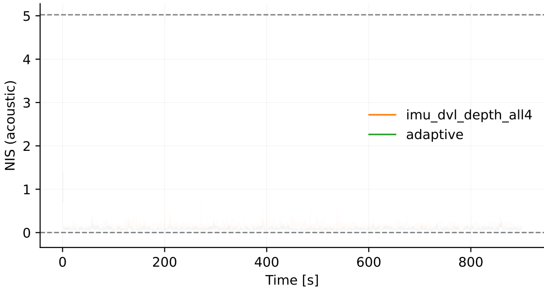
Acoustic NIS vs time (mean \pm 95% CI)
