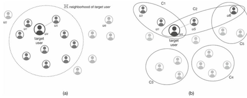
Figure 26 : Comparison between traditional neighborhood-based collaborative filtering (a) and community-based collaborative filtering (b) [50].
