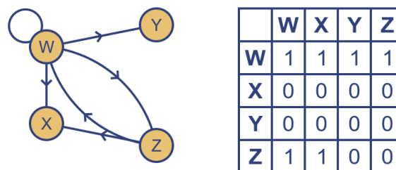
Figure 4 : Adjacency Matrix
