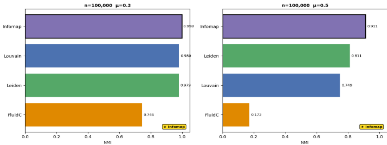
Figure 41 : LFR Benchmark Results: Network Size = 100000 nodes
