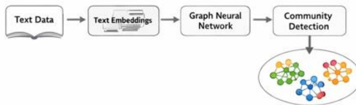
Figure 22 : Semantic-topological community detection framework
