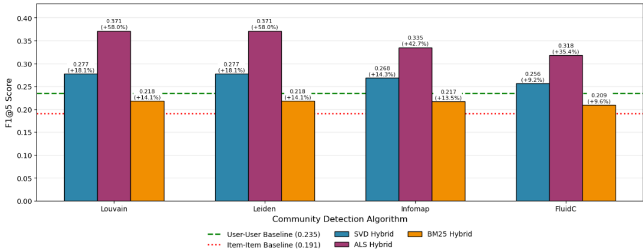
Figure 44 : Hybrid F1@5 scores vs community baselines.
