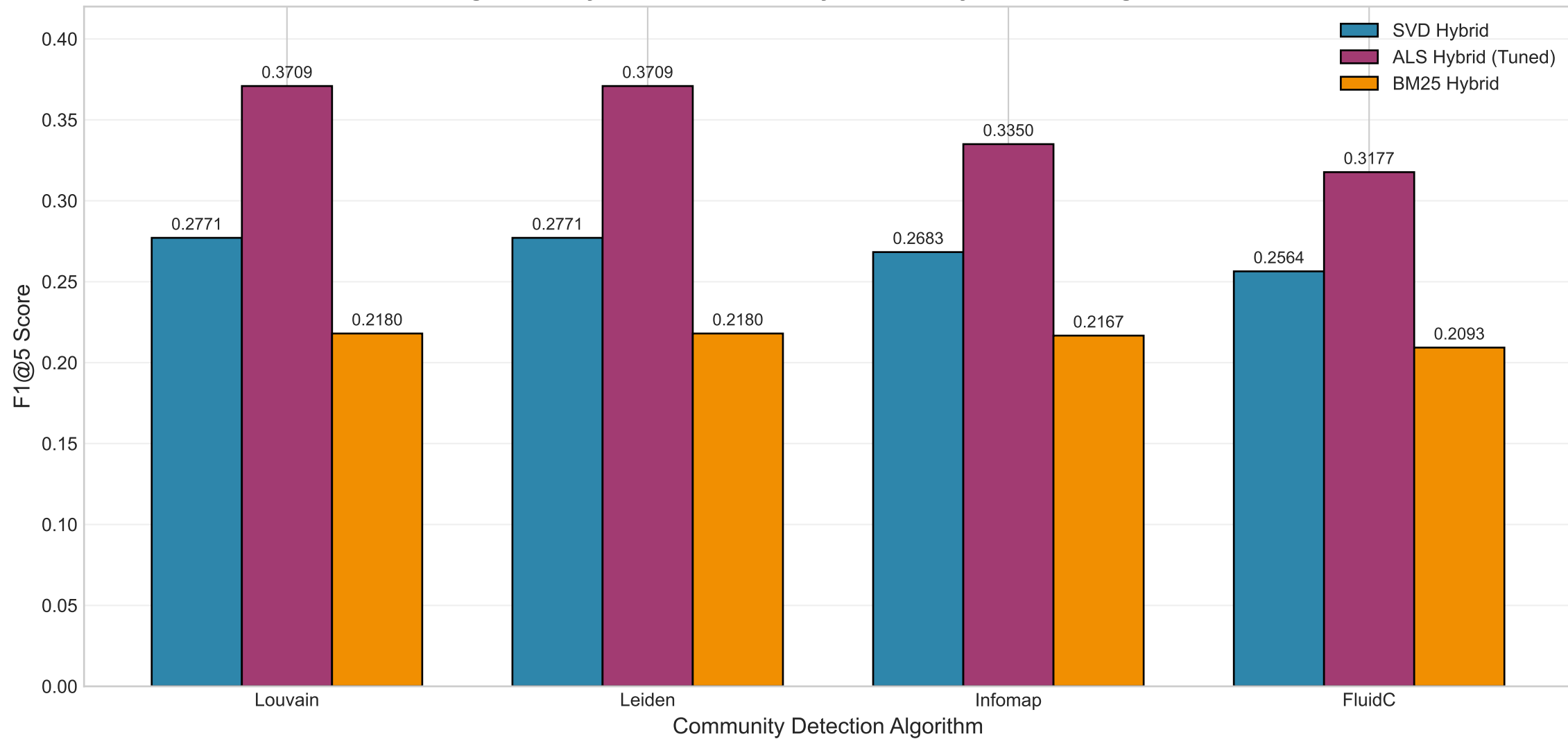
Figure 39: Hybrid Performance by Community Detection Algorithm
