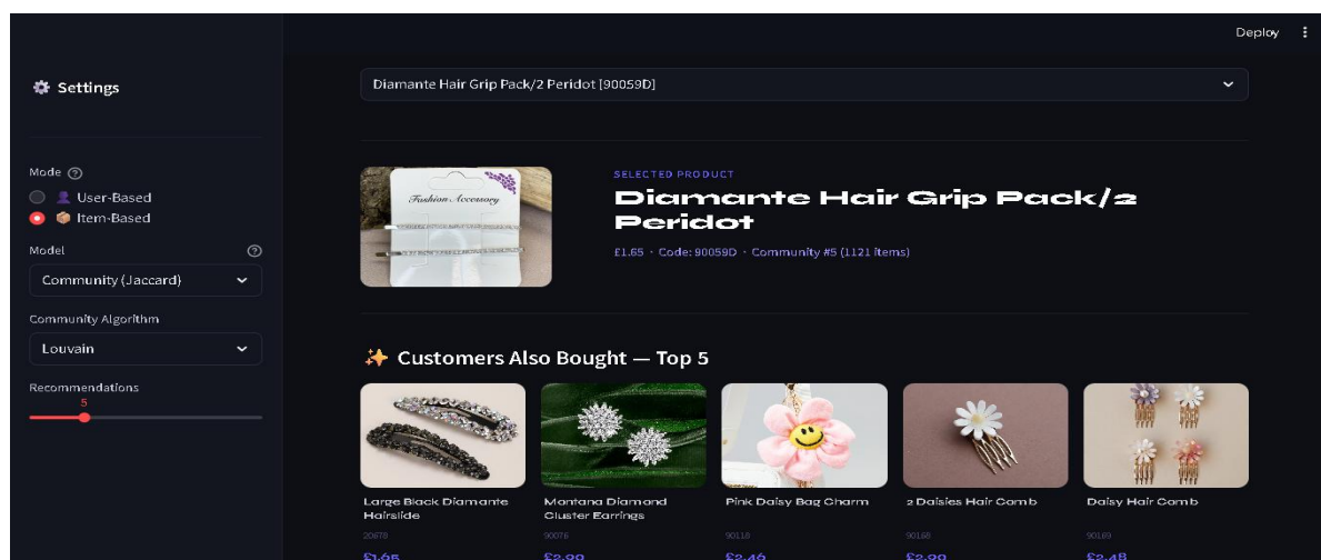
Figure 44 : Item-Based Interface
