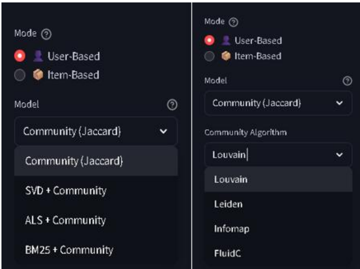
Figure 42 : Pipeline Configuration
