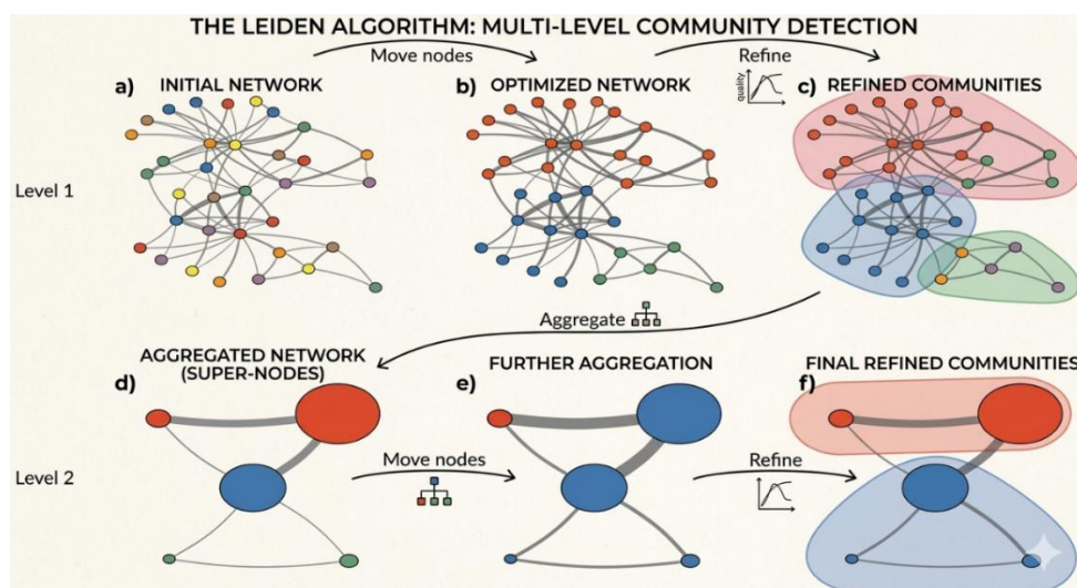
Figure 11 : Leiden Algorithm
