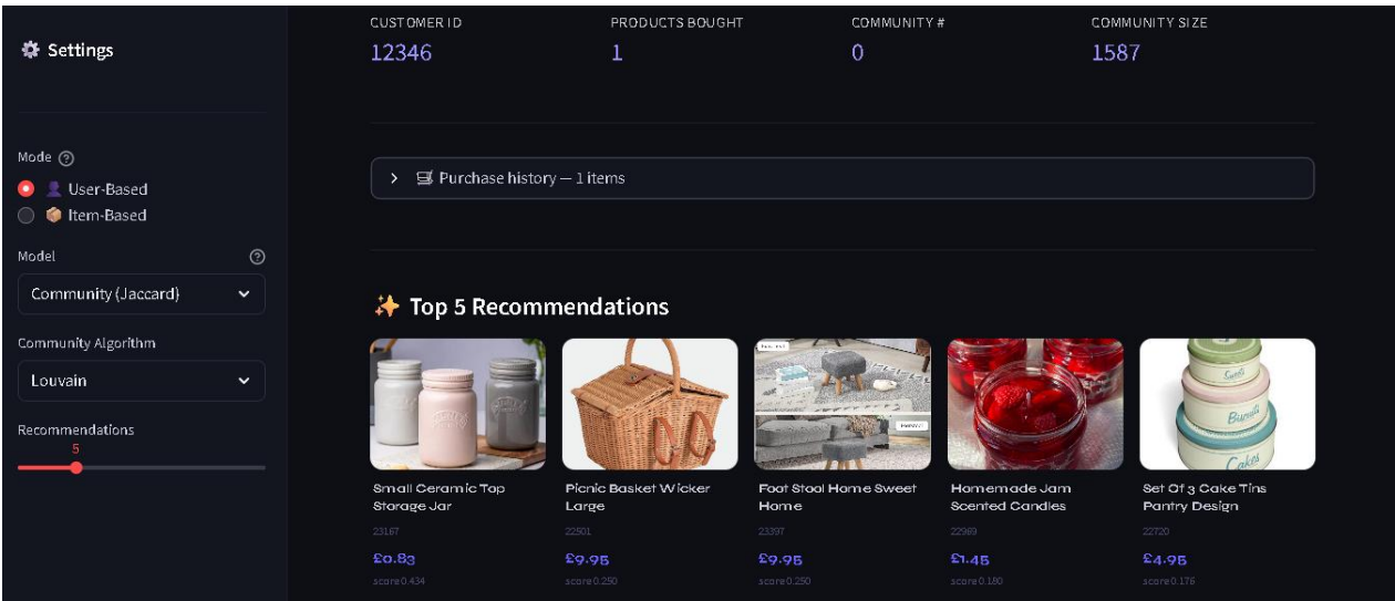
Figure 43 : User-Based Interface
