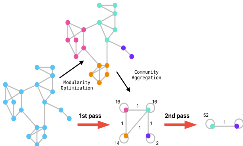
Figure 10 : Louvain Algorithm
