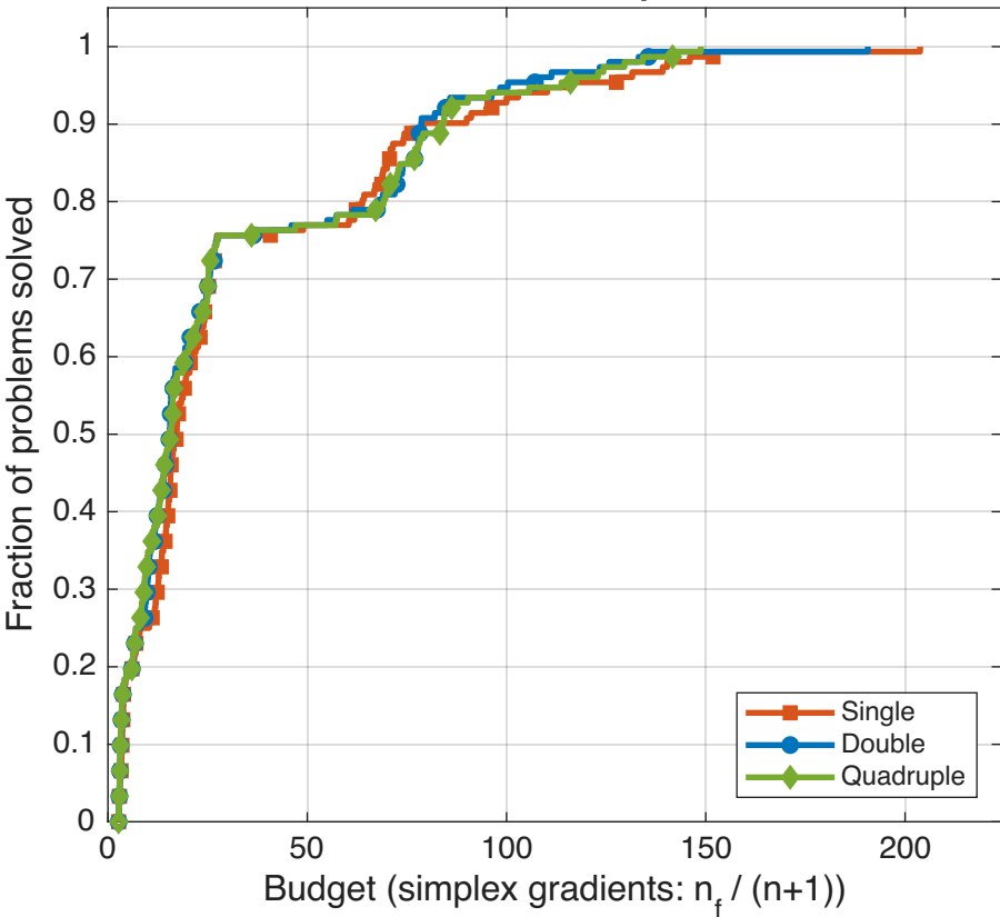
Data Profile — plain
