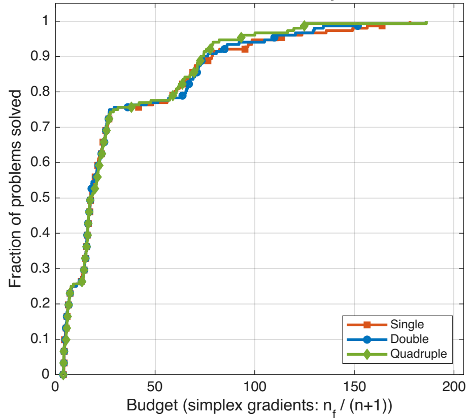
Data Profile — noisy
