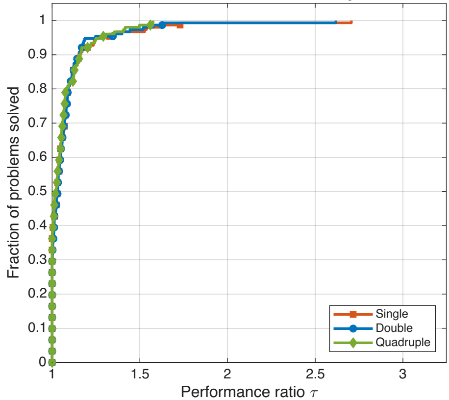
Performance Profile — noisy
