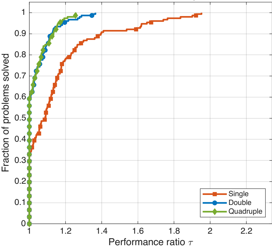
Performance Profile — plain
