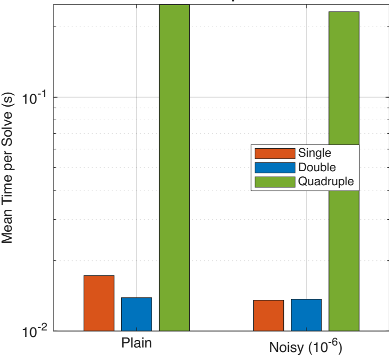
Time Comparison
