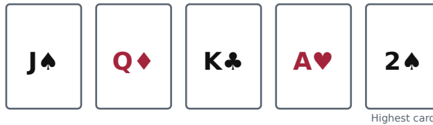
Run topped by a 2
