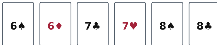
Chain of three pairs
