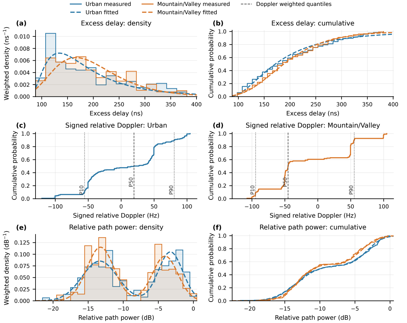
Fig. 2. Measured path-parameter distributions and fitted descriptions: (a)–(b) excess delay, (c)–(d) track-balanced empirical CDFs of signed relative Doppler for Urban and Mountain/Valley, respectively, and (e)–(f) relative path power. Fitted curves are shown for excess delay and relative power.
