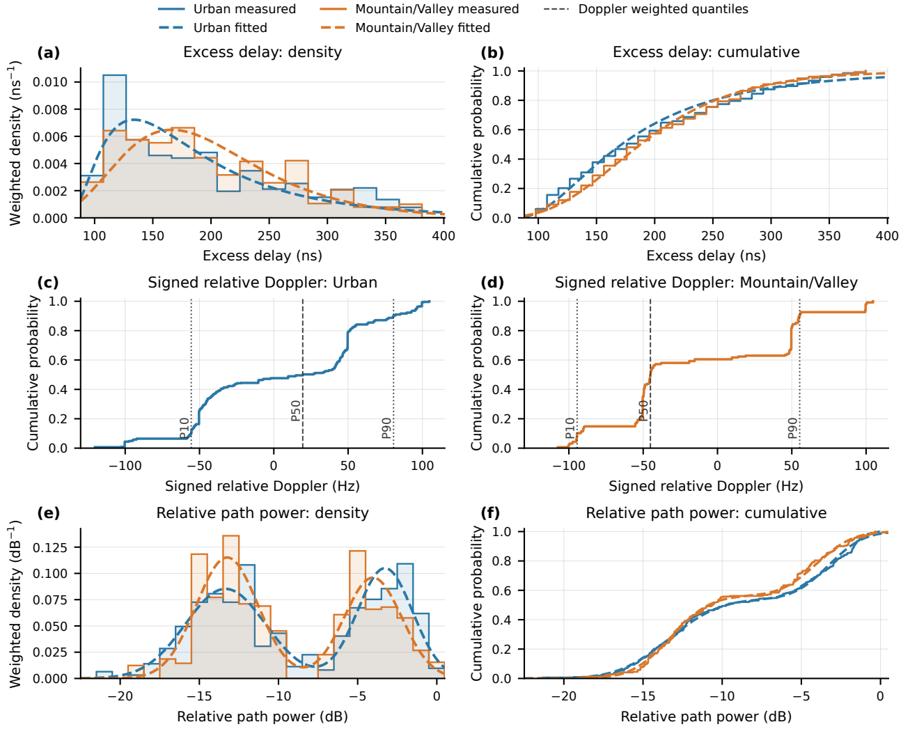
Fig. 2. Measured path-parameter distributions: excess delay (a,b), signed relative-Doppler ECDFs (c,d), and relative power (e,f) for Urban and Mountain/Valley.
