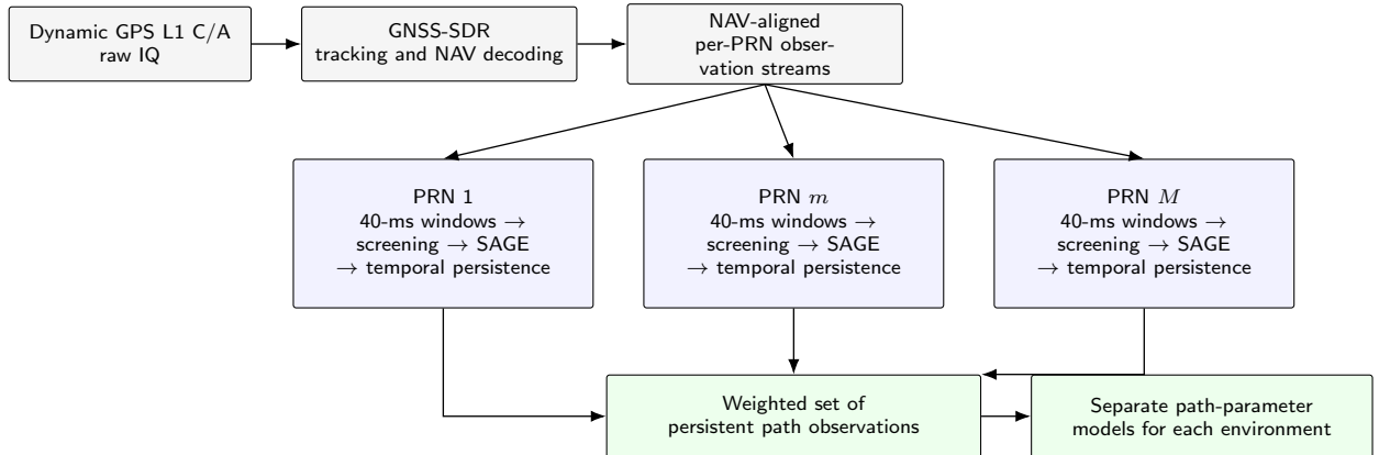
Fig. 1. Measurement and per-satellite MPC processing flow.
